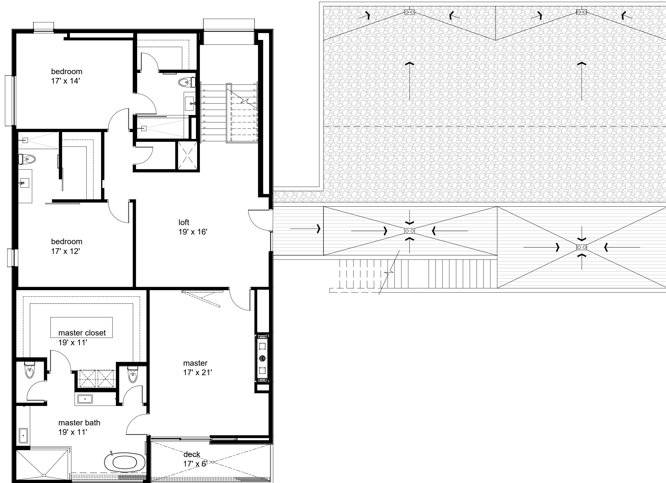
Model-A2 Level-2 Floor Plan 1/8"=1'-0"
